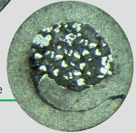
Cross-section of a seamed cored wire
