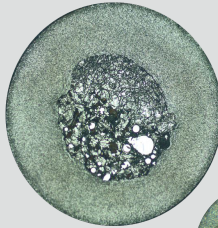
Cross-section of a seamed cored wire
